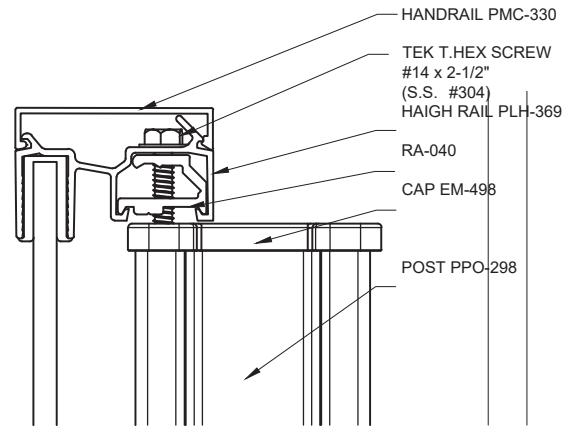
DETAIL A VIEW 1:2
